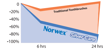
Reduction level of Streptococcus Mutans
